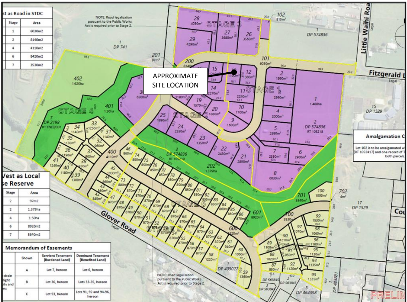
Figure 1-1: Existing Site Overview Plan - TRC GIS Maps
