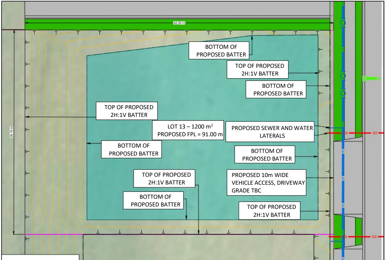
Figure 2-1: Lot 13 Site Information Plan Excerpt
